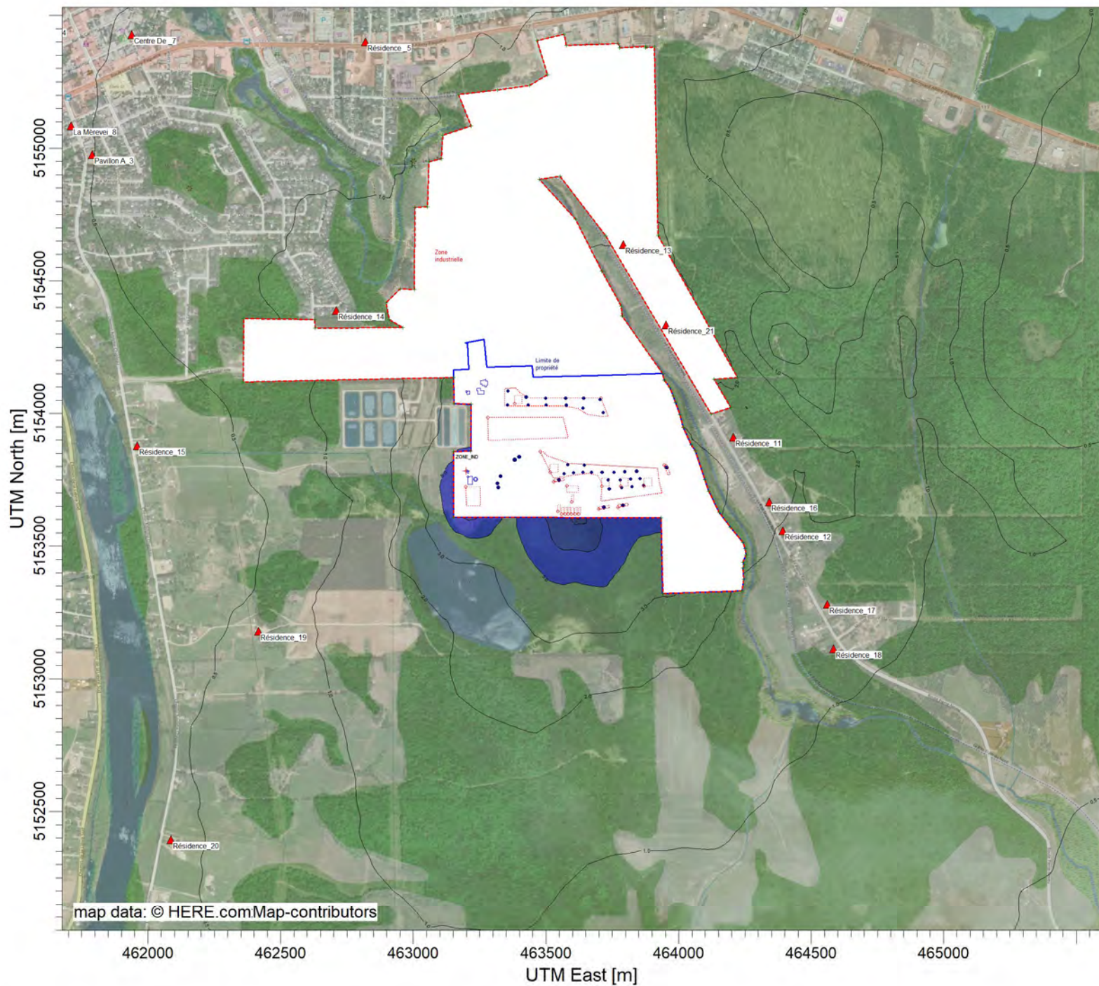
PLOT FILE OF 99.50TH PERCENTILE 1-HR VALUES FOR SOURCE GROUP: ALL Max: 58.0 [OU/M**3] at (463621.05, 5153608.77)
